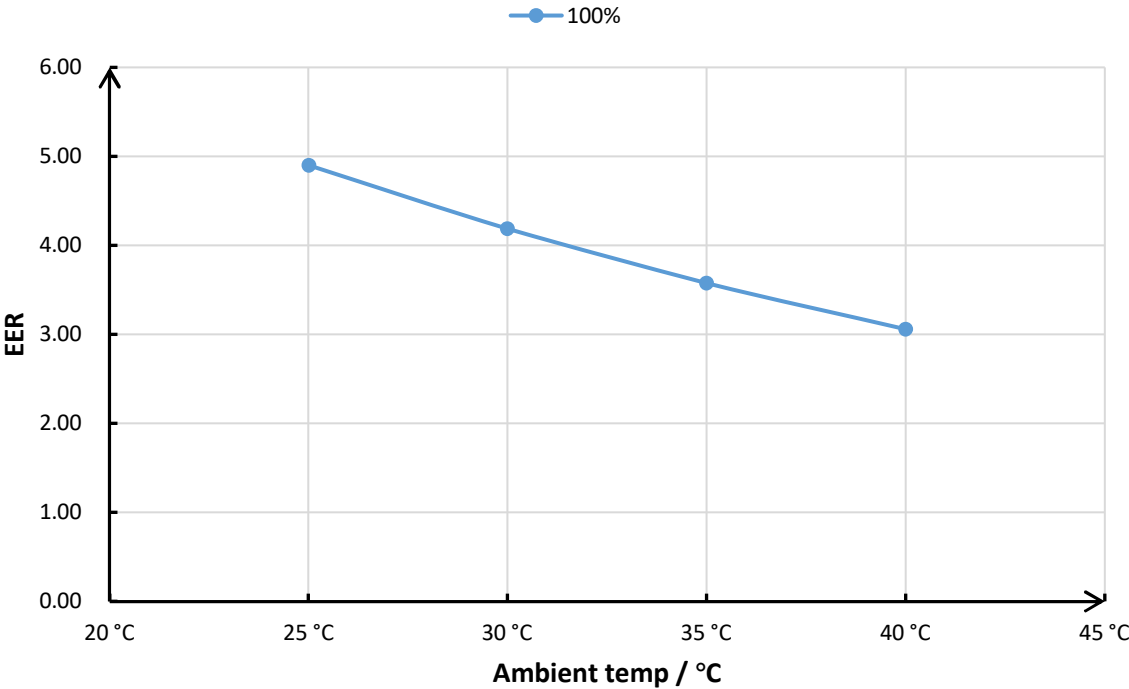
X20-32C EER Curve
