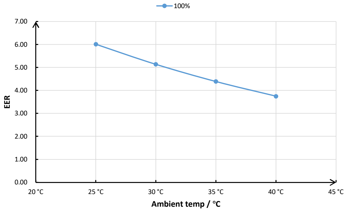
X20-22C EER Curve
