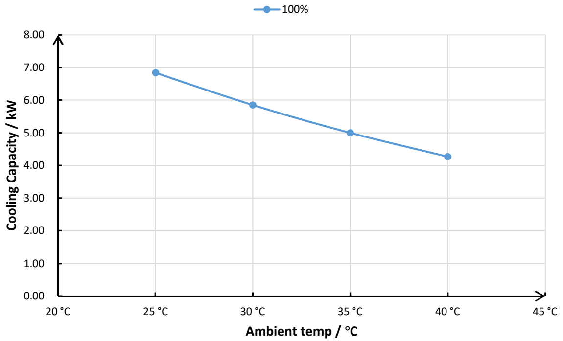
X20-11C Cooling Capacity Curve
