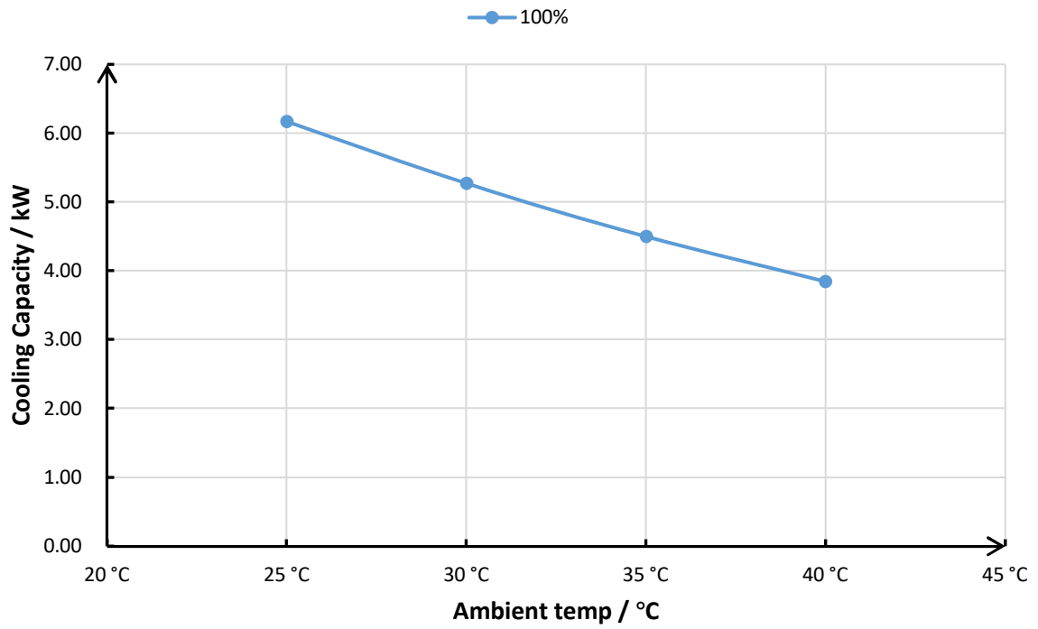
X20-09C Cooling Capacity Curve
