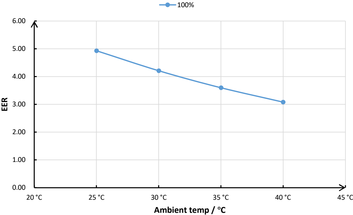
X20-26CT EER Curve
