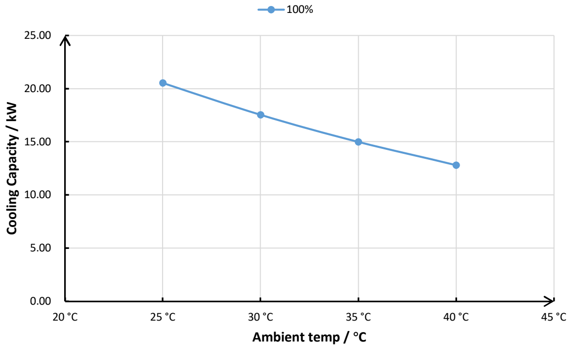
X20-32C Cooling Capacity Curve
