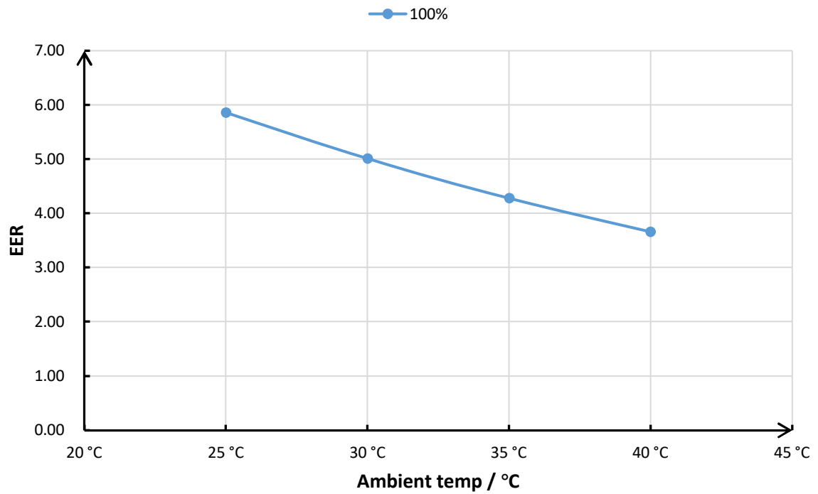
X20-16C EER Curve
