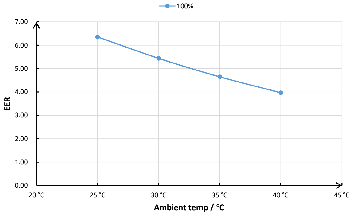
X20-09C EER Curve
