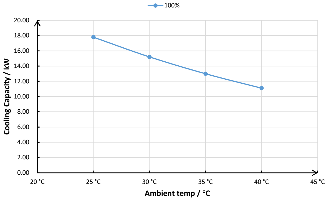
X20-26C Cooling Capacity Curve
