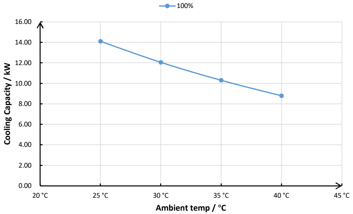
X20-18C Cooling Capacity Curve
