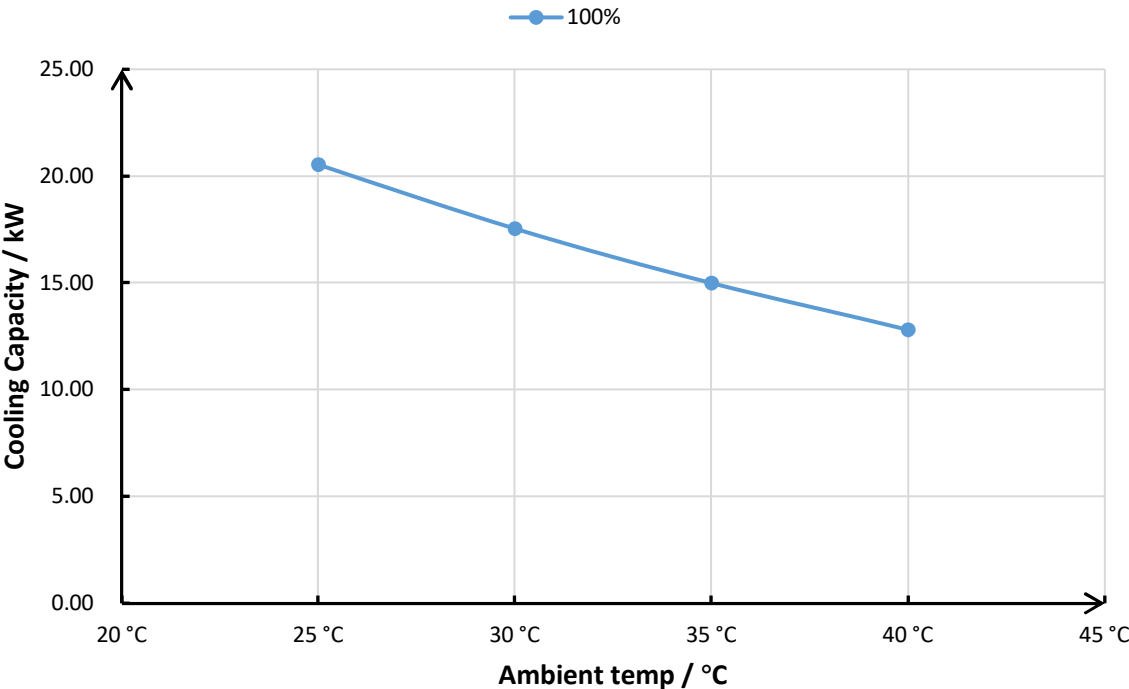
X20-32CT Cooling Capacity Curve
