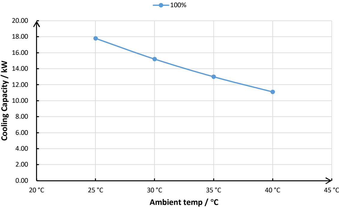
X20-26CT Cooling Capacity Curve
