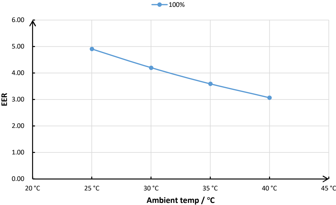
X20-40CT EER Curve
