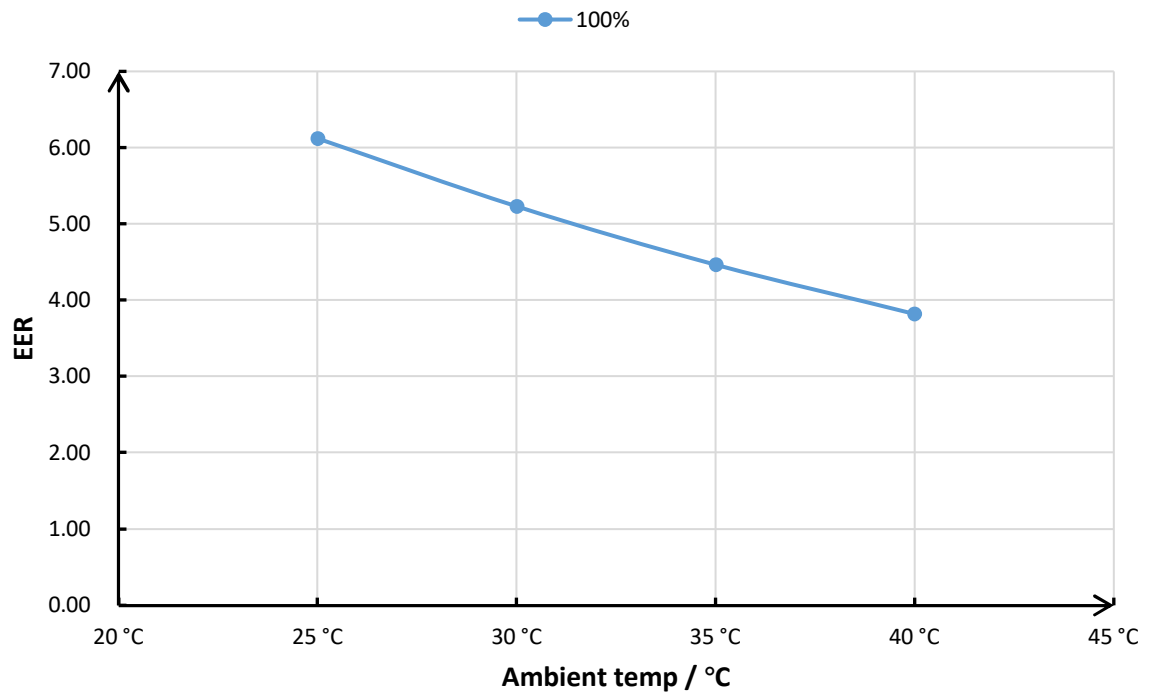
X20-14C EER Curve
