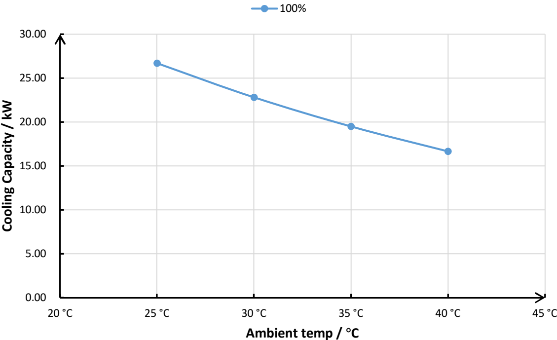
X20-40CT Cooling Capacity Curve
