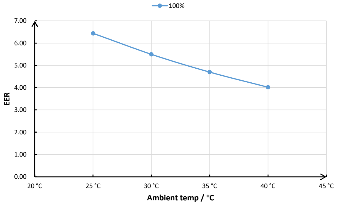
X20-11C EER Curve
