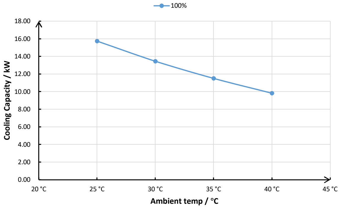
X20-22C Cooling Capacity Curve
