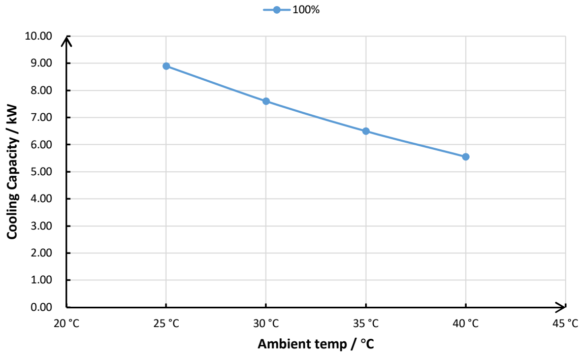
X20-14C Cooling Capacity Curve
