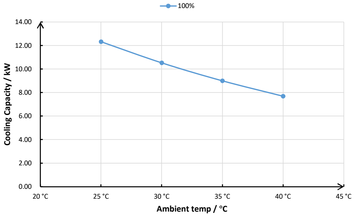
X20-16C Cooling Capacity Curve
