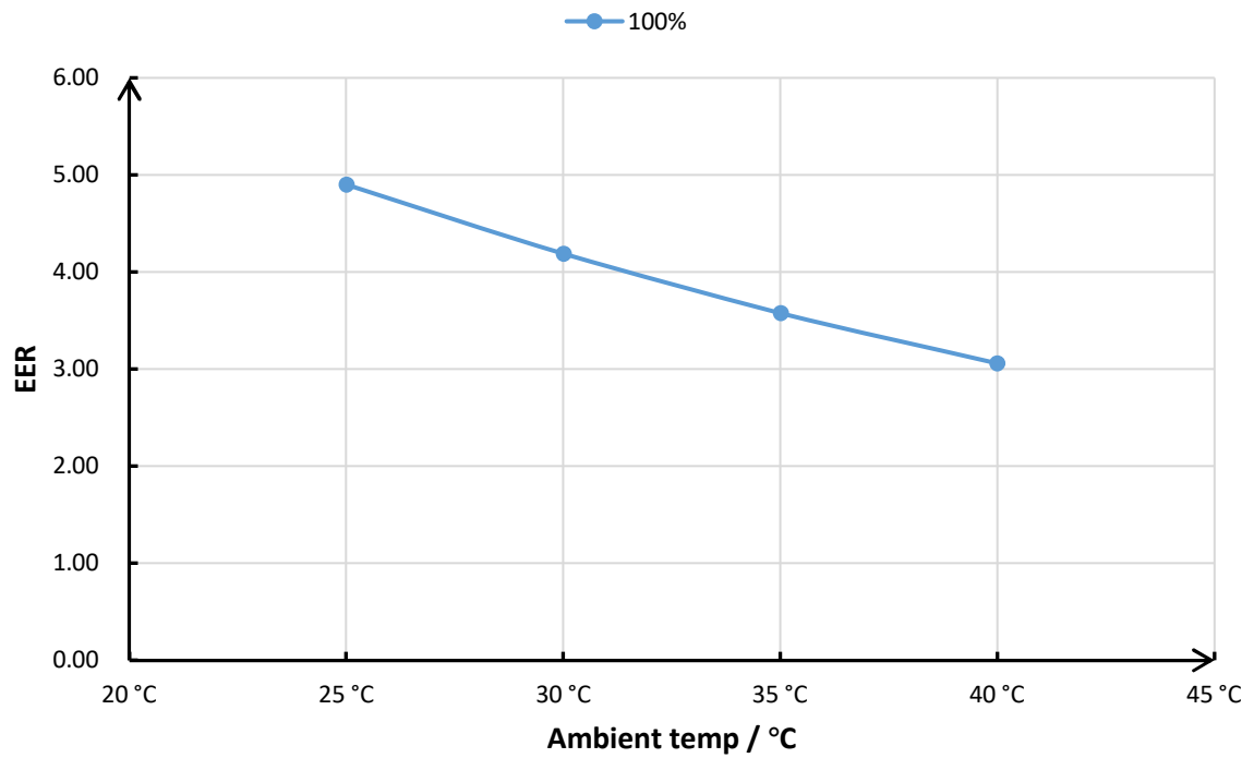
X20-32C EER Curve
