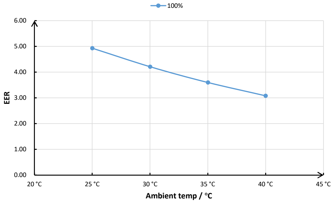
X20-26C EER Curve
